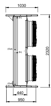
VISTA FRONTAL
