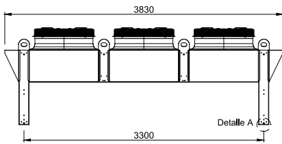
Vista Principal
